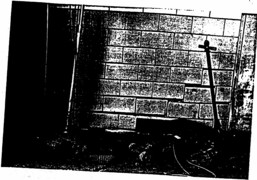
PHOTO S-10 Diagonal masonry cracking at settled foundation - interior.
