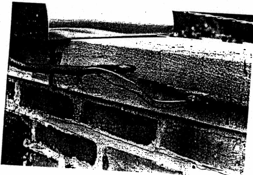
PHOTO E-5 Eroded conduits and exposed wiring on roof of west building.
