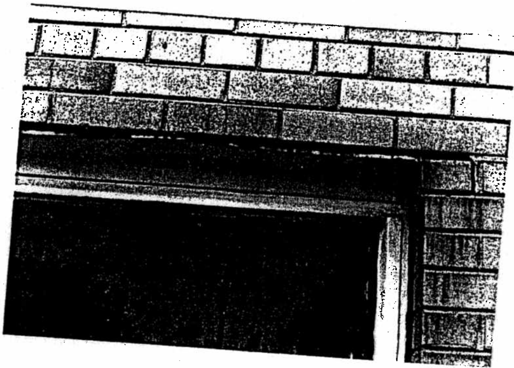
PHOTO S-6 Buckled lintel flanges (close-up).
