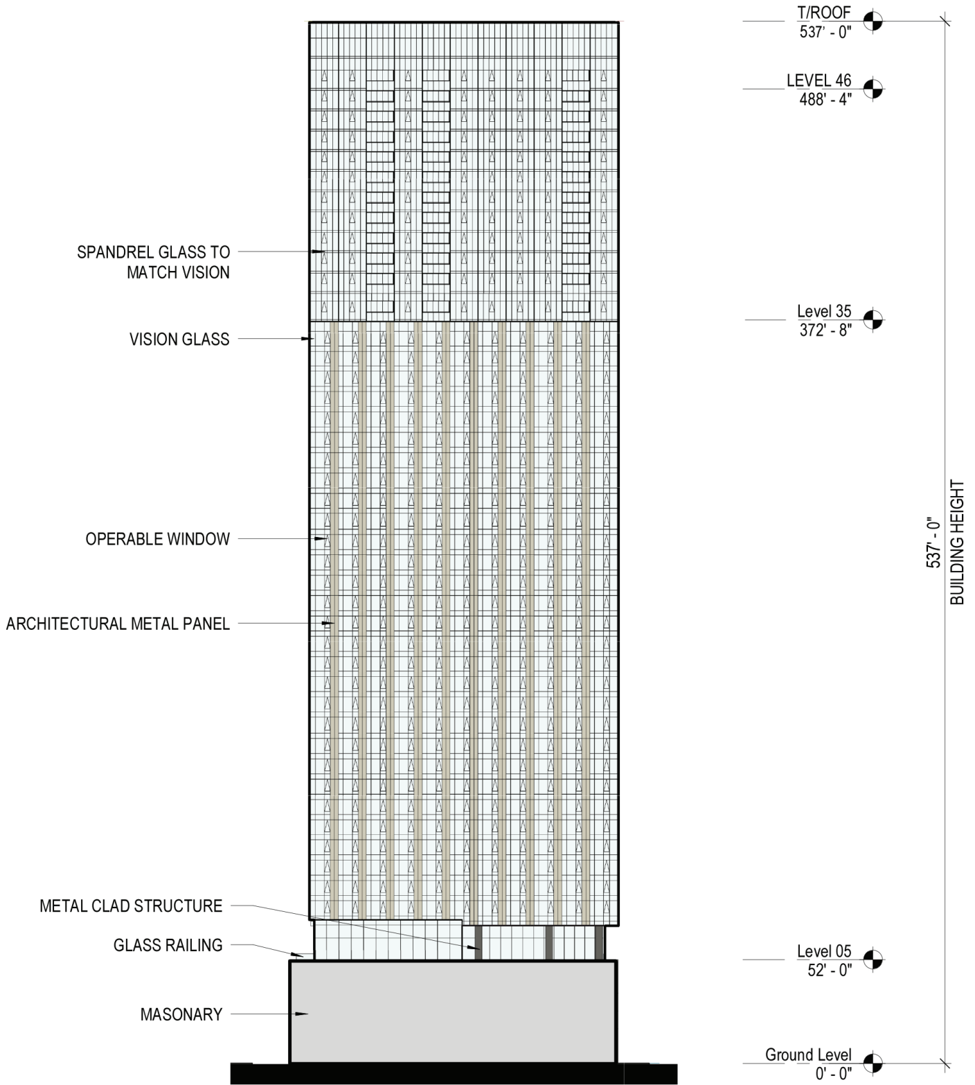
WEST BUILDING ELEVATION Scale: 1" = 50'-0"
