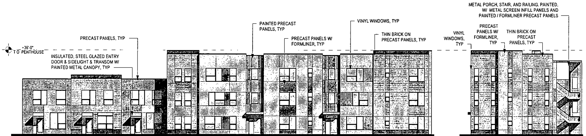
BUILDING 20 WEST ELEVATION
