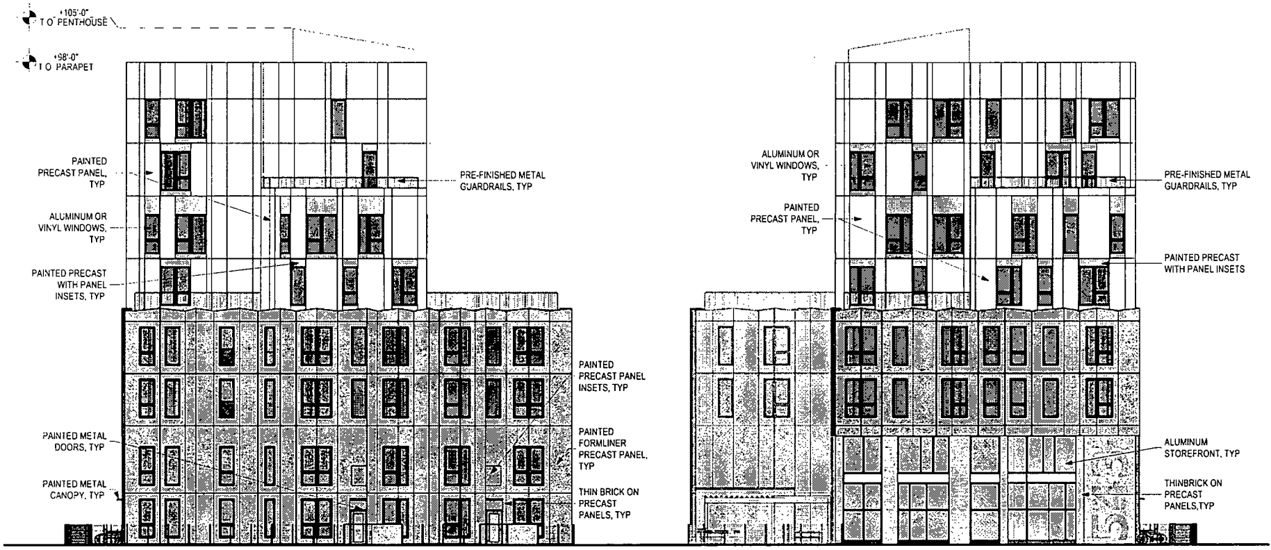
BUILDING 22 EAST ELEVATION
