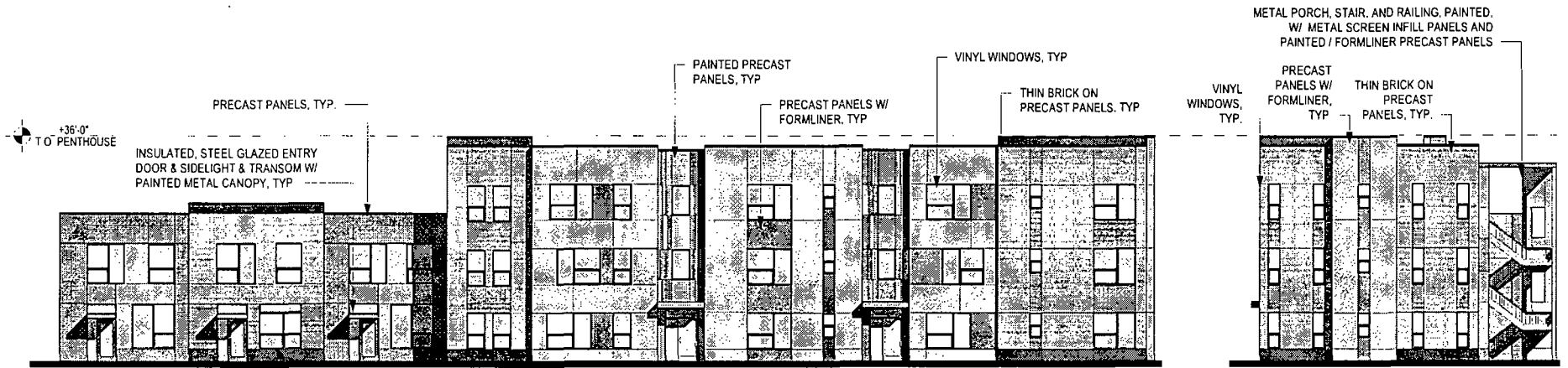
BUILDING 21 EAST ELEVATION
