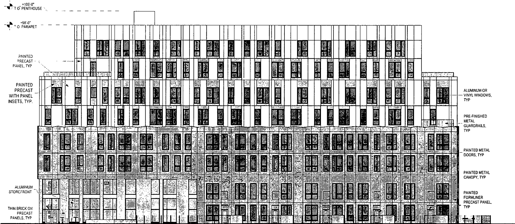
BUILDING 22 SOUTH ELEVATION
