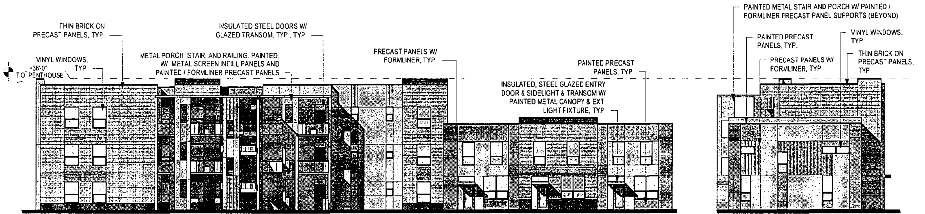
BUILDING 21 WEST ELEVATION
