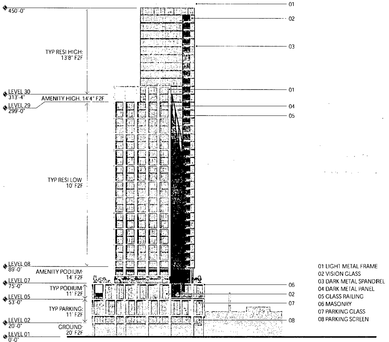
NORTH ELEVATION
